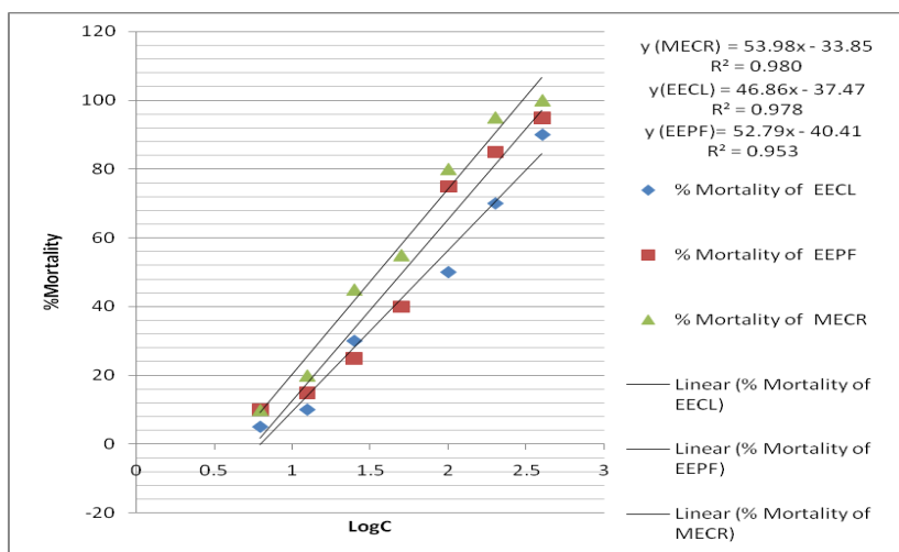
Fig 1: Determination of \text{LC}_{50} value for EECL, EEPF and MECR from linear correlation between log concentrations versus % Mortality.
