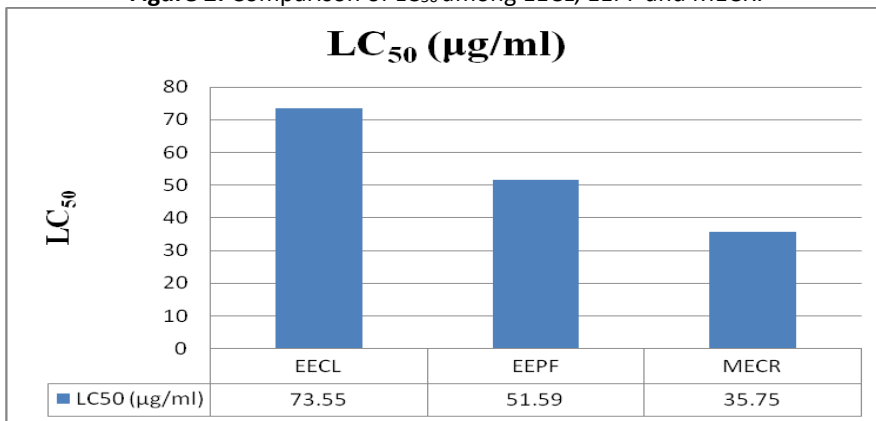
Figure 2: Comparison of \text{LC}_{50} among EECL, EEPF and MECR.
