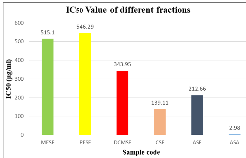
Fig 2: Comparison of IC 50 values for different fraction
