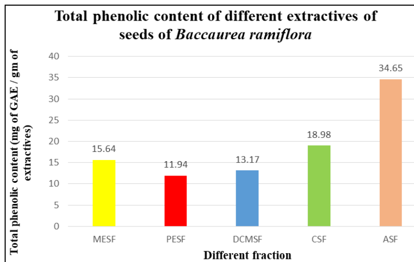
Fig 3: Graphical representation of total phenolic content (mg of GAE/ gm of extractives) of different extractives of seeds of Baccaurea ramiflora .
