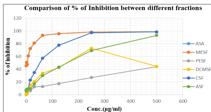
Fig 1: Result for DPPH radical scavenging assay of Baccaurea ramiflora .
