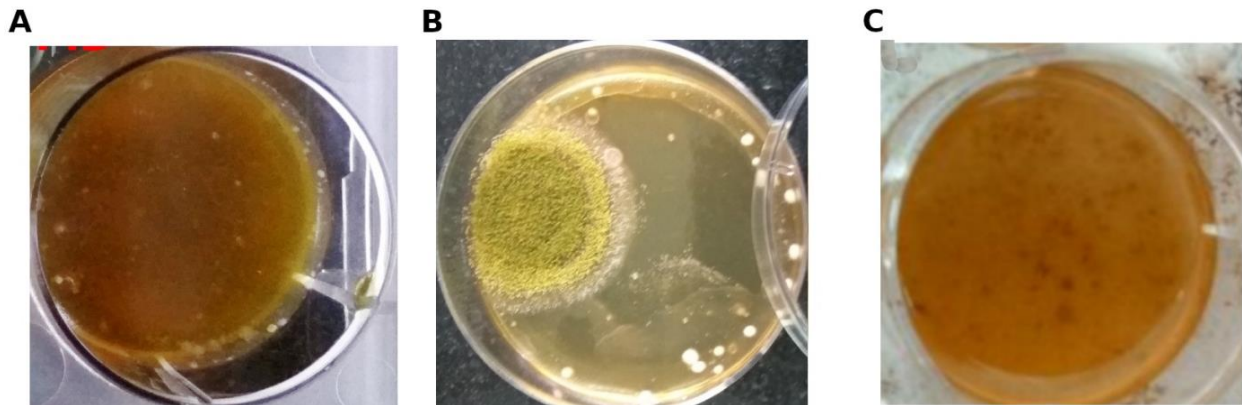
Fig 7: Antifungal activity
