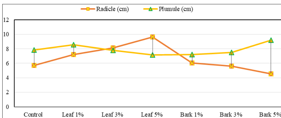
Fig 1: Reduction/stimulation percentage of radicle and plumule growth over control.
